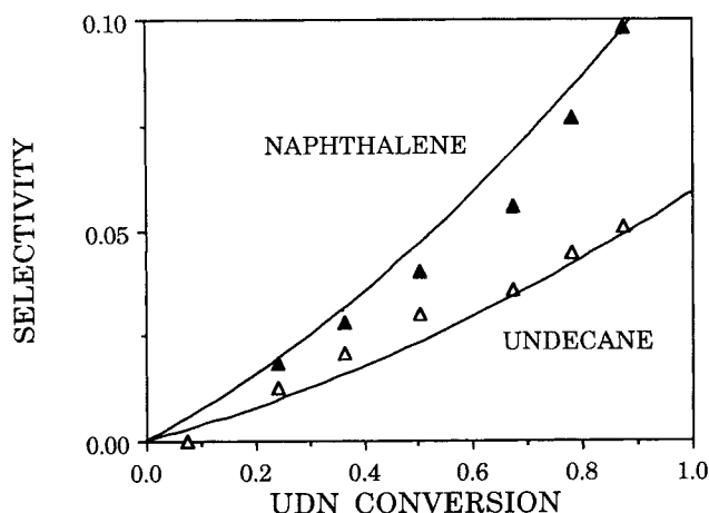
Figure 7c. UDN selectivity to major products (naphthalene and dodecane).
